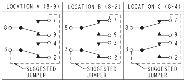
SPIT SCHEMATIC USE R2XXXX7XXXX FOR (8-9),(8-2),(8-4) USE R2XXXX74XXXX FOR (OFF),(8-2),(8-4) USE R2XXXX67XXXX FOR (8-9),(8-2),(OFF)
